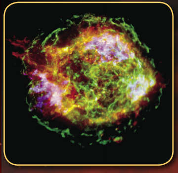
Cassiopeia A
