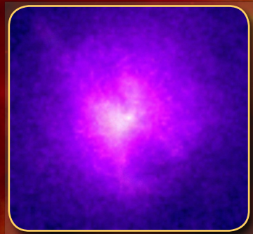
Hydra A
