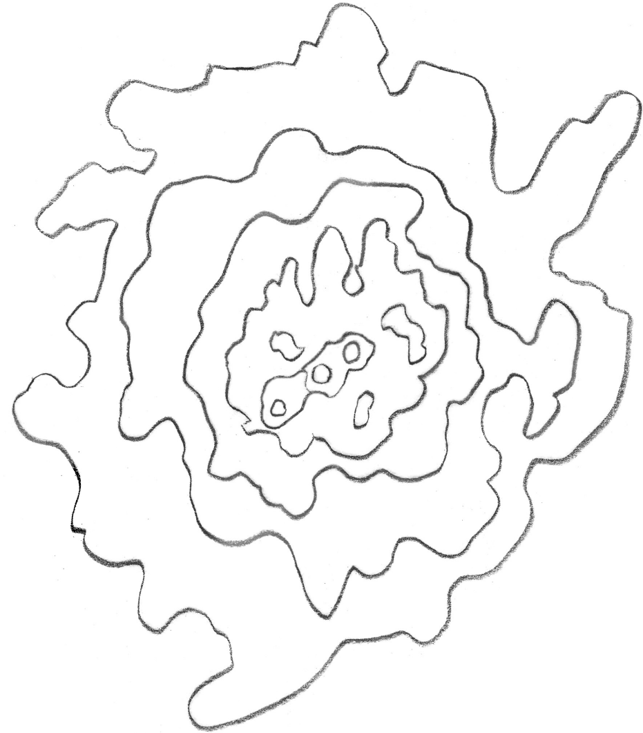
Galaxy Clusters: 3C295
