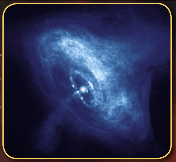
Crab Nebula
