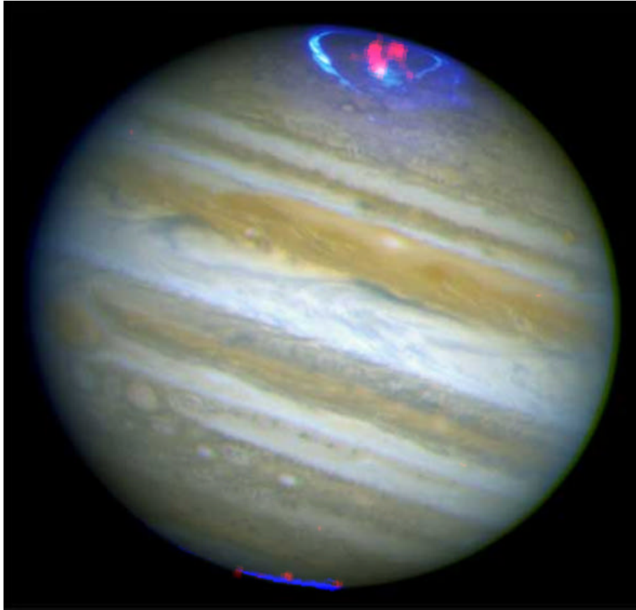
X-ray/UV/Optical
