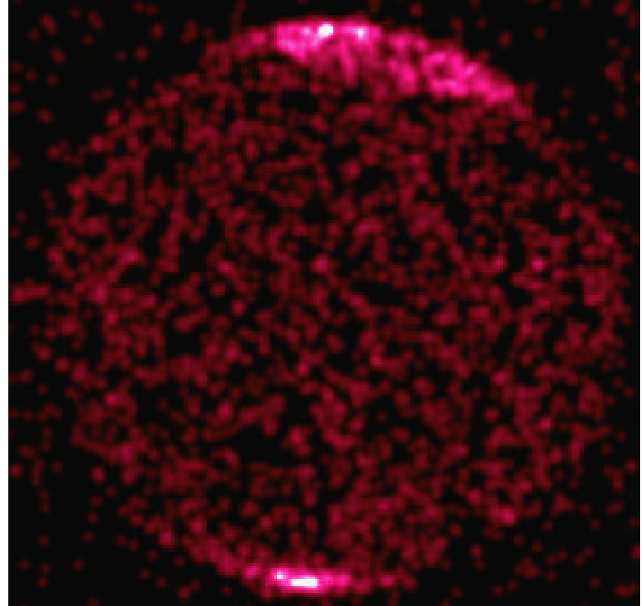
X-ray
