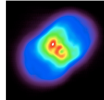
Infrared
