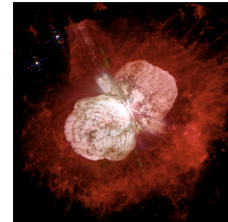
Optical
