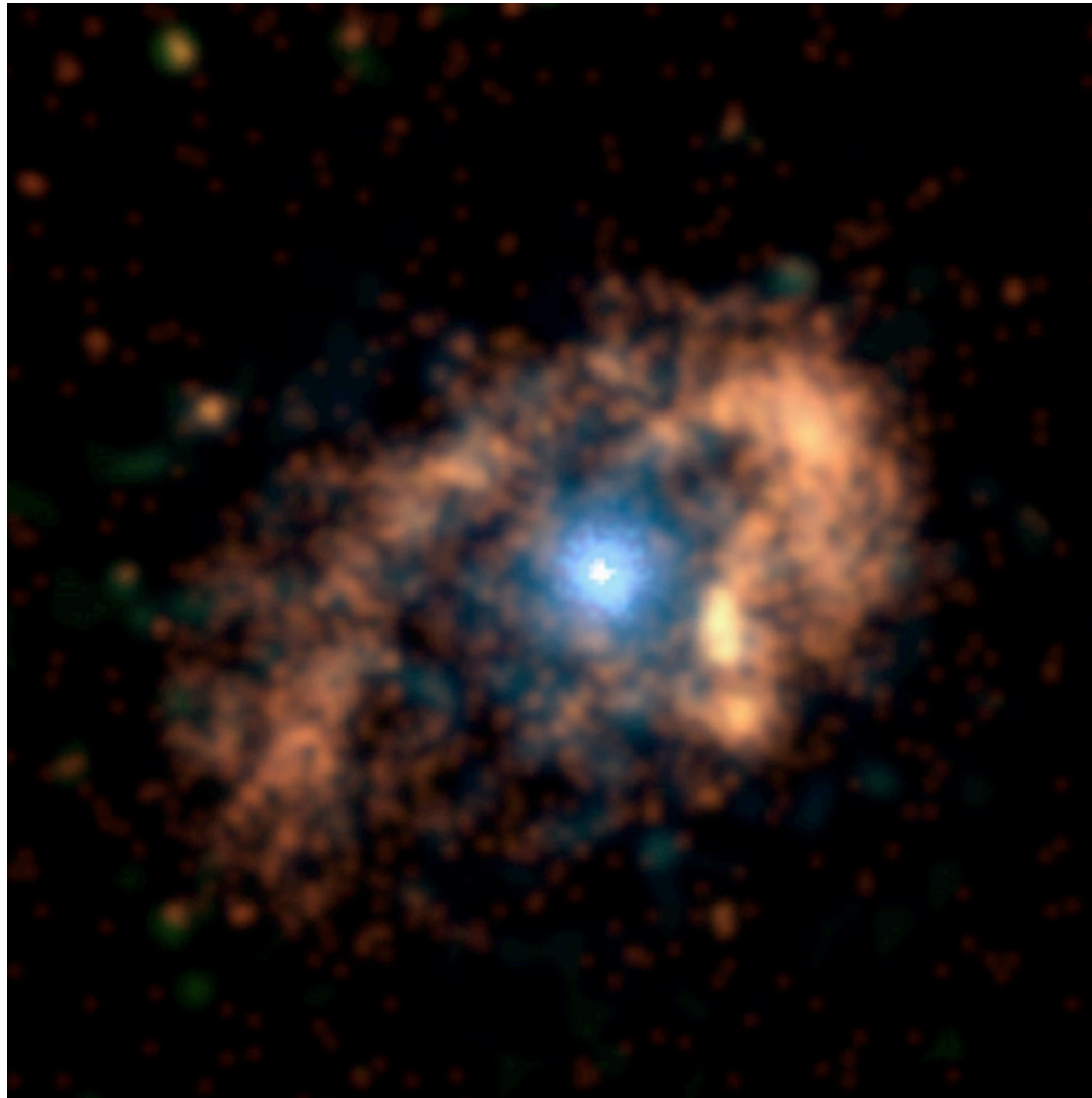
X-ray
