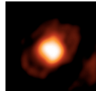
Radio
