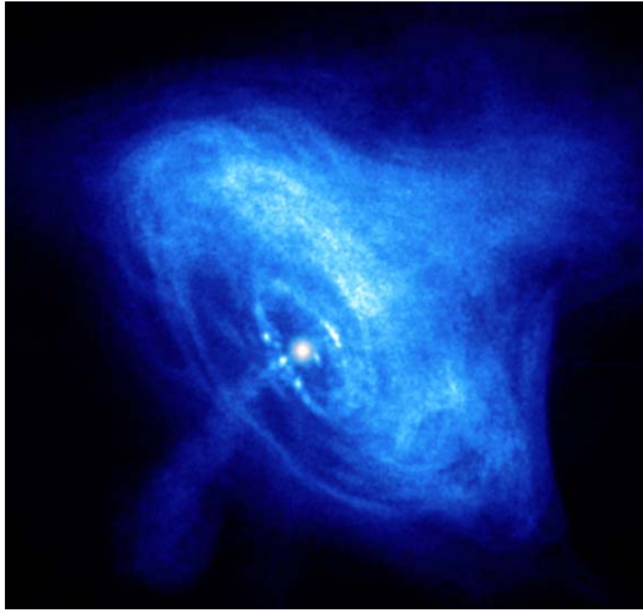
Crab Nebula
